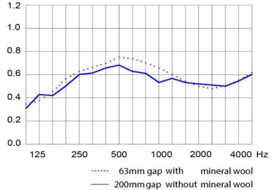
Absorption according to EN ISO 354
